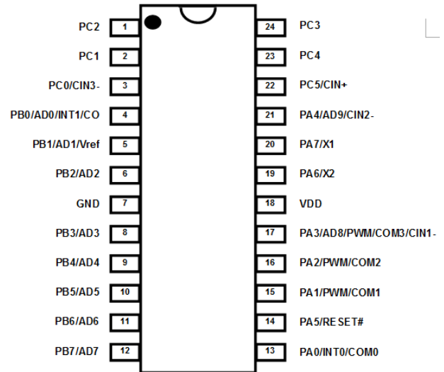
PTB0234XXS-S24 (SOP24-300mil) PTB0234XXS-K24 (Skinny DIP24-300mil)
