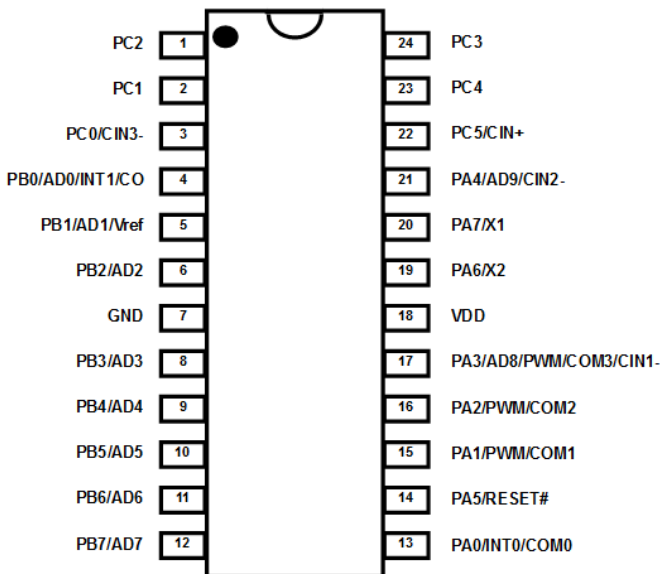
PTB0234XXS-S28 (SOP28-300mil) PTB0234XXS-K28 (Skinny DIP28-300mil)
