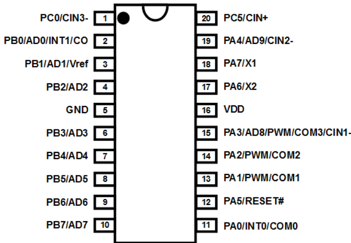
PTB0234XXS-S20 (SOP20-300mil) PTB0234XXS-D20 (DIP20-300mil)
