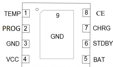
DFN2*2-8L
