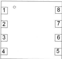
DFN2*2-8L
